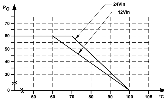
FIGURE 2. Typical derating curve
