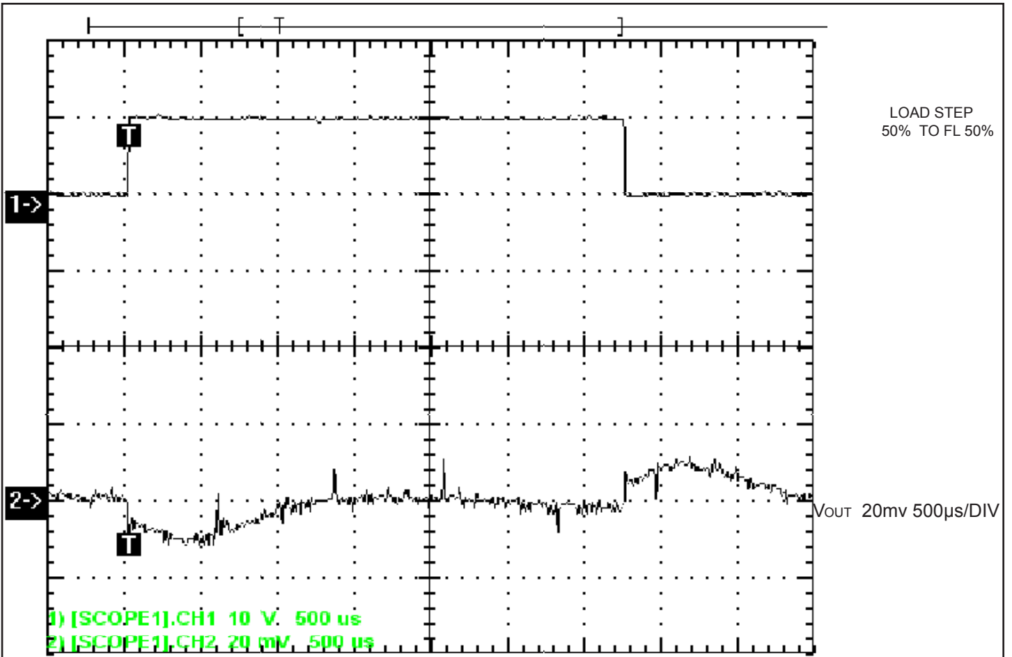
FIGURE 2.TRANSIENT RESPONSE
