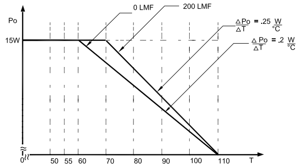
FIGURE 3. Derating of BDH10018
