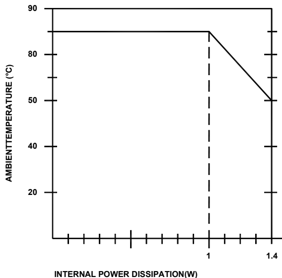
FIGURE 2. Derating curve
