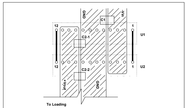
Solder side
