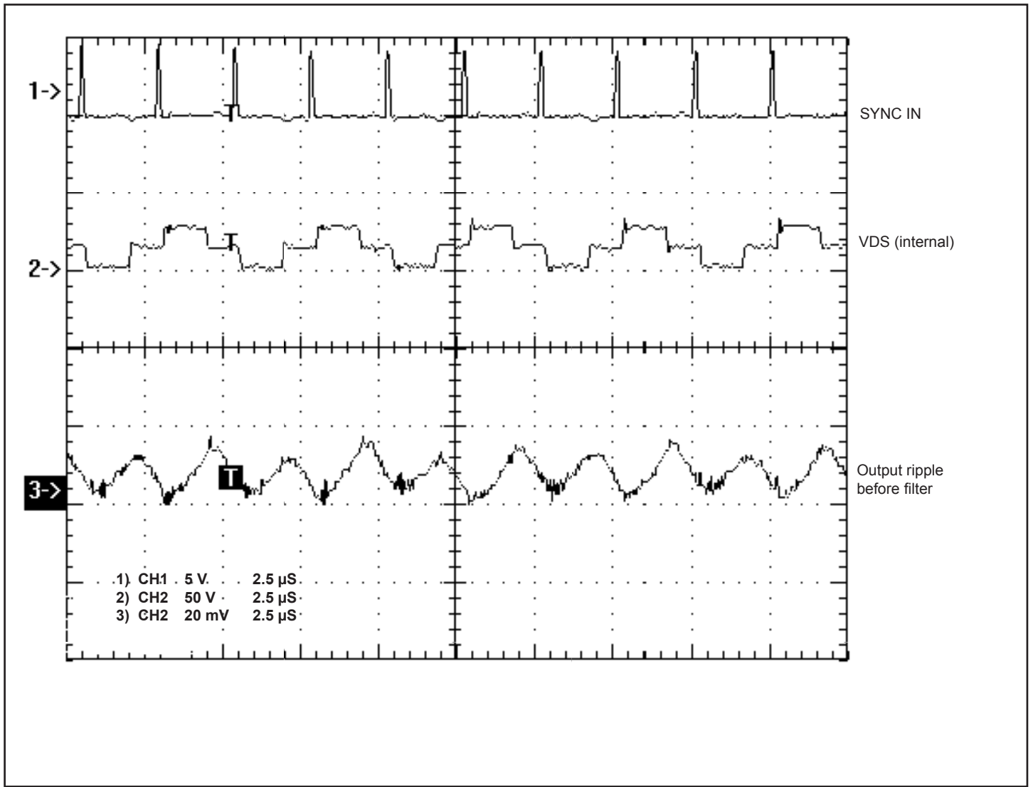
FIGURE 7. External Synchronization
