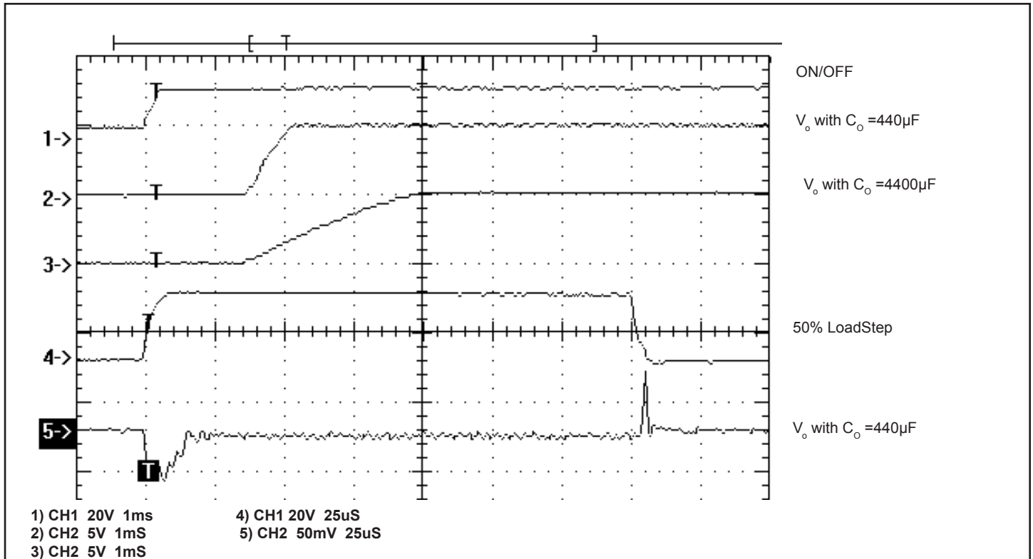
FIGURE 3. EAL50S5/24 Turn on delay with soft start and transient response
