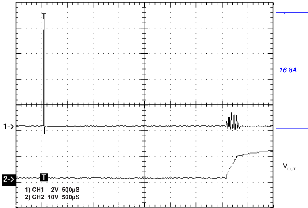
FIGURE 5A. (CH1) Inrush current without hot pluggable circuit ON V IN 48V, Current spike duration 5μS
