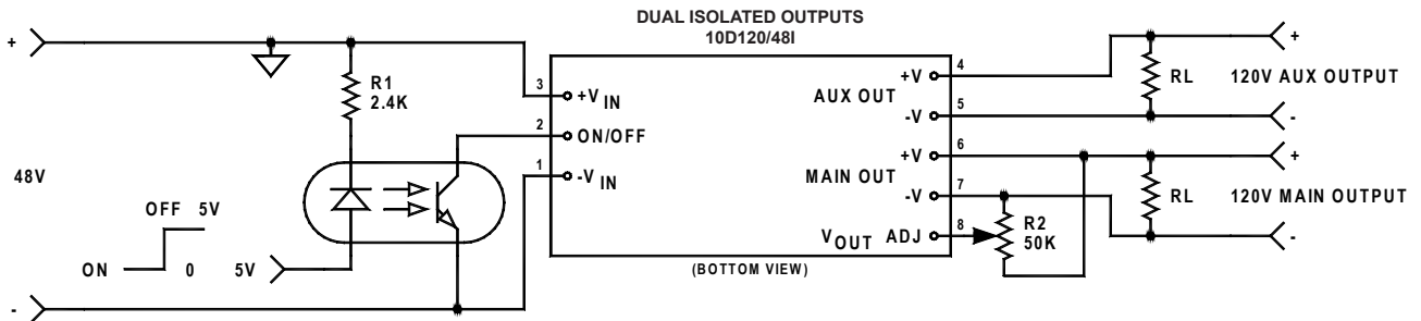
FIGURE 3. Dual isolated output connection diagram
