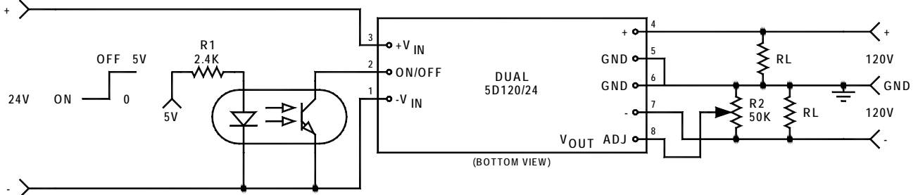
FIGURE 2. Dual connection diagram
