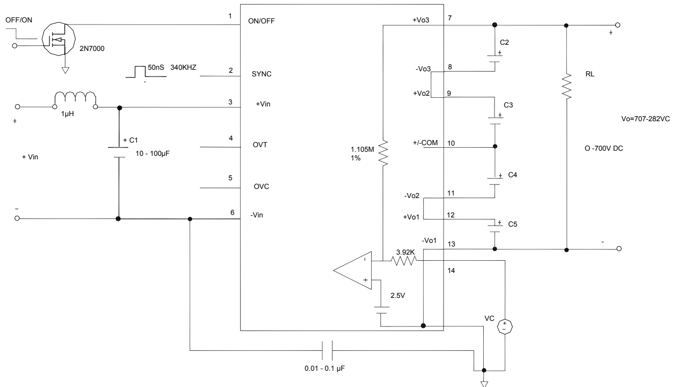
FIGURE 1. Typical Output Diagram Connection of AVH50 Series Single Output 0 to 700V Output
