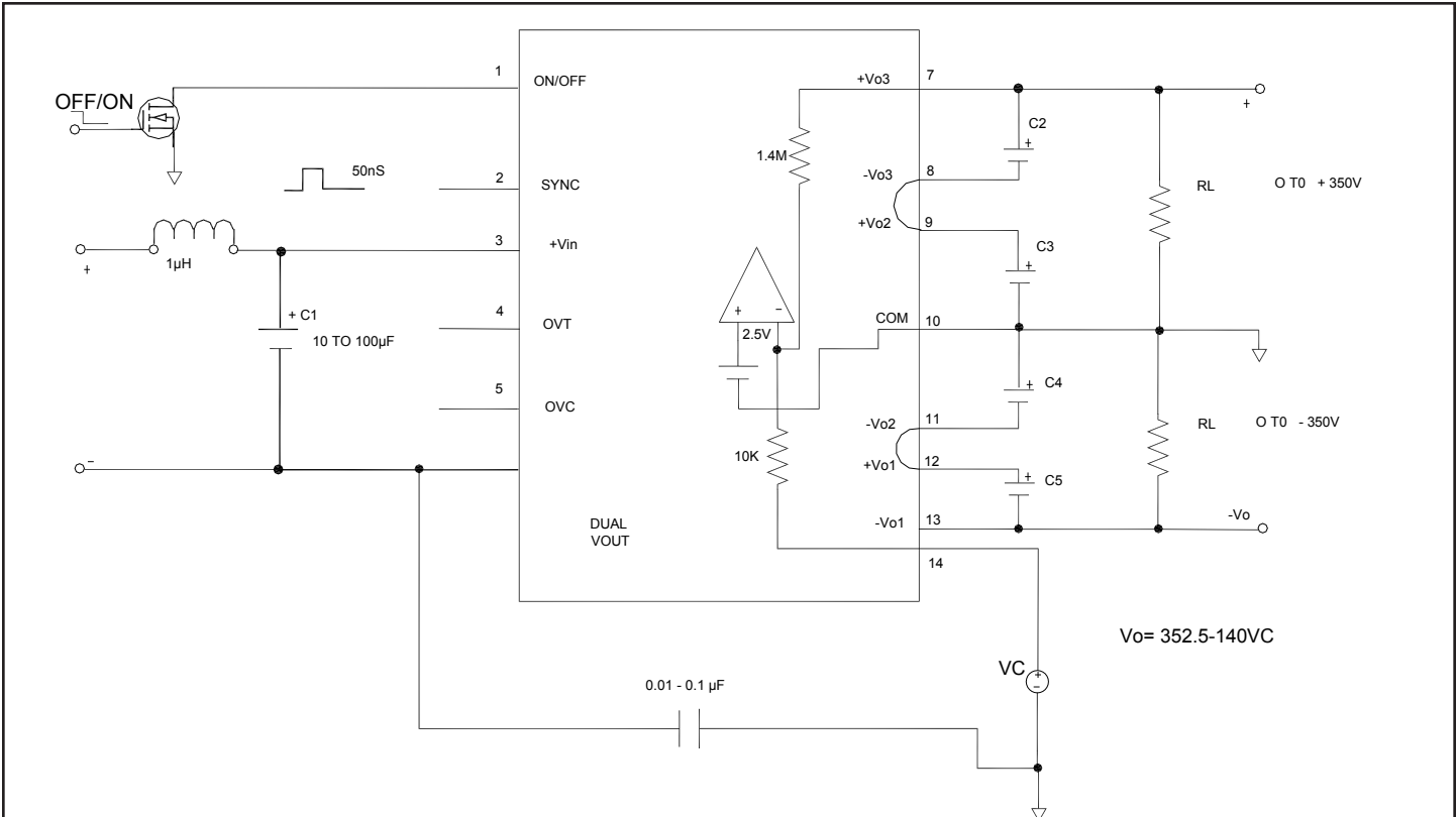
FIGURE 2. Typical Output Diagram Connection of AHV 50 Series Dual Output \pm 350V Max V_C = 0 TO 2.5V V_{OUT} = 350 TO 0V NOTE: For -40^\circ Operation C2 Through C5 Must Be 3.3 \mu F Or Greater @ 200V X7R Or Y5U Type Example: Nippon Chemi-Con (TCD51E2E155M)
